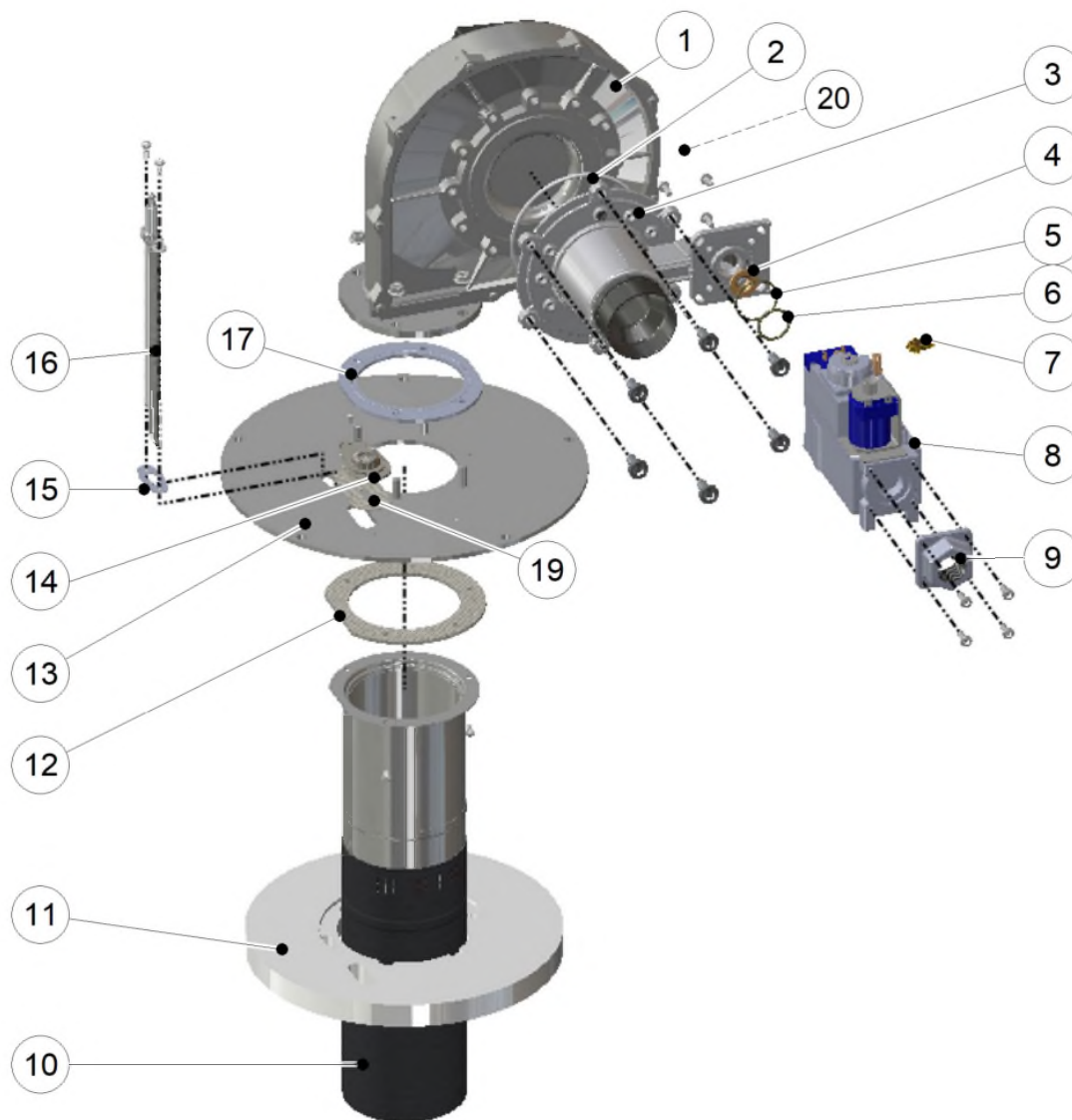
Burner HM120TC
