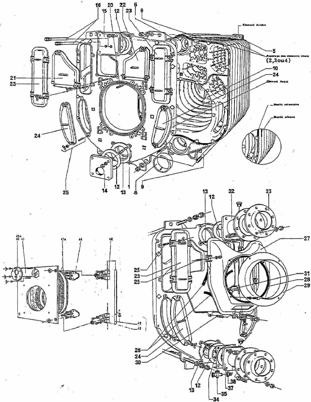
1622 CORPS CHAUDIERE IDEAL 2400
