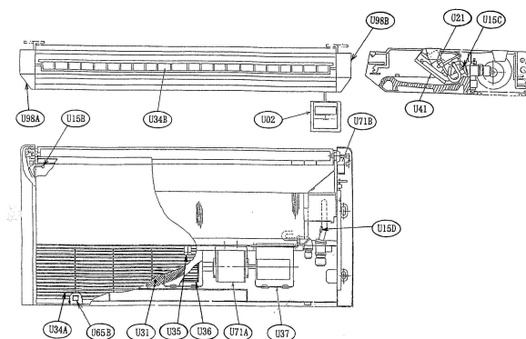
LOCATION OF SPARE PARTS IN THE UNIT A MODEL: RPC-2.5FS
