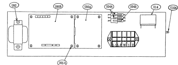
LOCATION OF ELECTRICAL EQUIPMENT IN THE ELECTRICAL BOX
