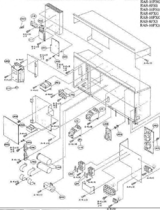
LOCATION OF ELECTRICAL EQUIPMENT IN THE ELECTRICAL BOX
