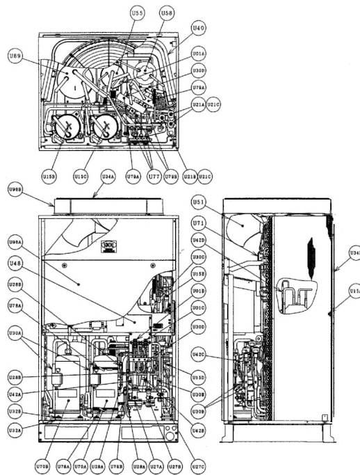
LOCATION OF SPARE PARTS IN THE UNIT A MODEL: RAS-10FX3
