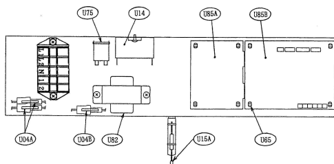
LOCATION OF ELECTRICAL EQUIPMENT IN THE ELECTRICAL BOX
