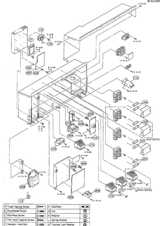
LOCATION OF ELECTRICAL EQUIPMENT IN THE ELECTRICAL BOX MODEL : RAS-16FS3 RAS-20FS3
