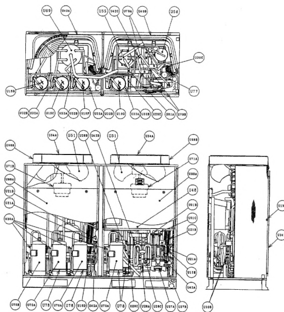
LOCATION OF SPARE PARTS IN THE UNIT A MODEL: RAS-20FS3
