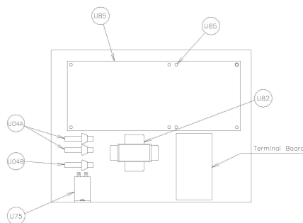
LOCATION OF ELECTRICAL EQUIPMENT IN THE ELECTRICAL CONTROL BOX
