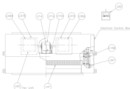
LOCATION OF SPARE PARTS IN THE UNIT FOR MODEL: RPI-2AG6E, RPI-2.5AG6E, RPI-3AG6E and RPI-3.5AG6E
