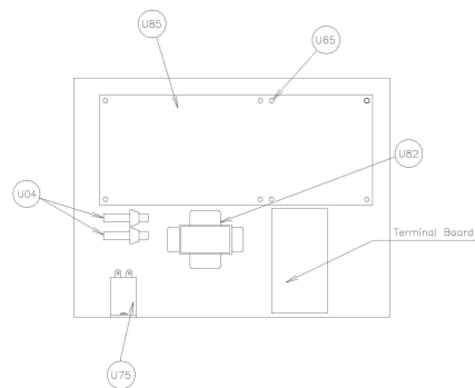
LOCATION OF ELECTRICAL EQUIPMENT IN THE ELECTRICAL CONTROL BOX
