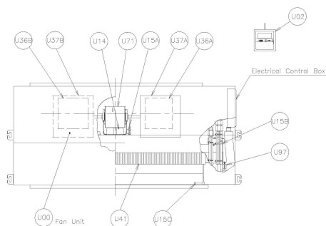
LOCATION OF SPARE PARTS IN THE UNIT FOR MODEL: RPI-2HQ5E, RPI-2.5HQ5E, RPI-3HQ5E and RPI-3.5HQ5E
