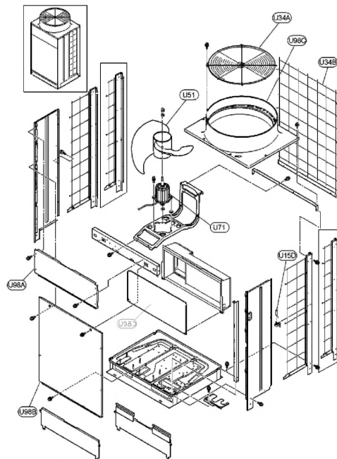
CABINET AND FAN
