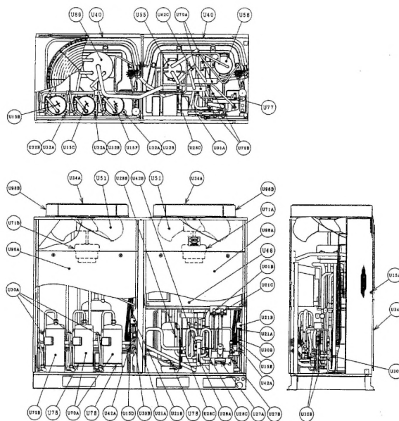
LOCATION OF SPARE PARTS IN THE UNIT A MODEL: RAS-16FS3
