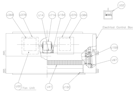
LOCATION OF SPARE PARTS IN THE UNIT FOR MODEL: RPI-2HG6E, RPI-2.5HG6E, RPI-3HG6E and RPI-3.5HG6E
