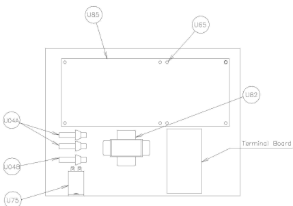
LOCATION OF ELECTRICAL EQUIPMENT IN THE ELECTRICAL CONTROL BOX
