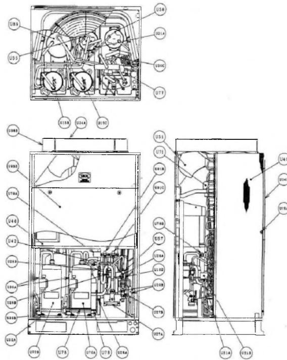
LOCATION OF SPARE PARTS IN THE UNIT A MODEL: RAS-10FSG
