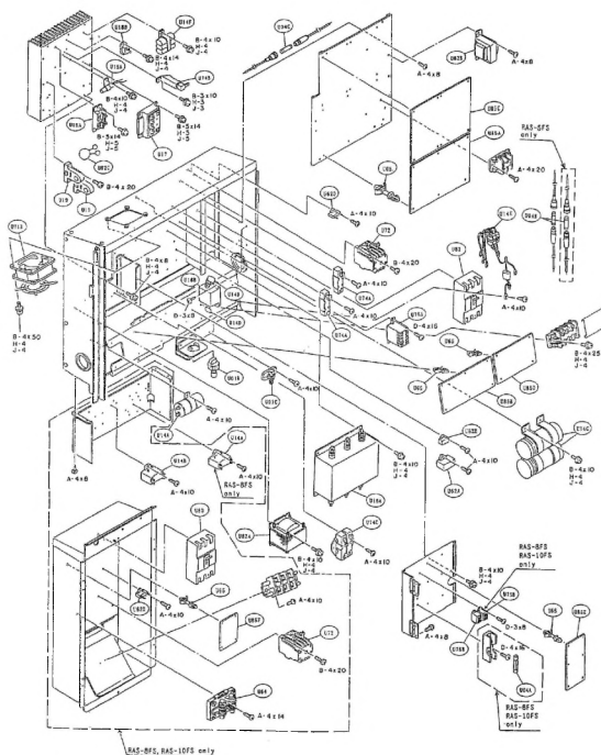
LOCATION OF ELECTRICAL EQUIPMENT MODELS: RAS-5FS IN THE ELECTRICAL BOX RAS-8FS RAS-10FS
