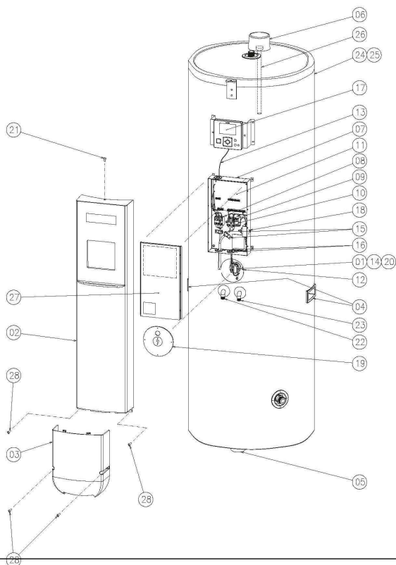
LOCATION OF SERVICE PARTS IN THE UNIT
