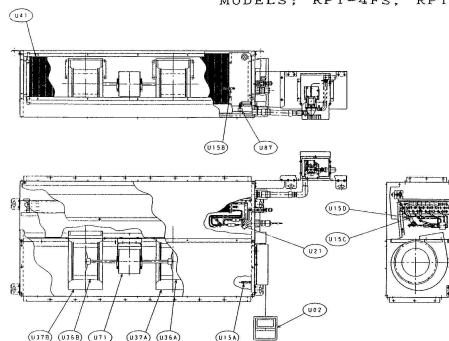
LOCATION OF ELECTRICAL EQUIPMENT IN THE ELECTRICAL BOX
