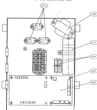
LOCATION OF ELECTRICAL EQUIPMENT IN THE ELECTRICAL BOX
