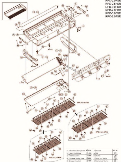
LOCATION OF SERVICE PARTS IN THE UNIT
