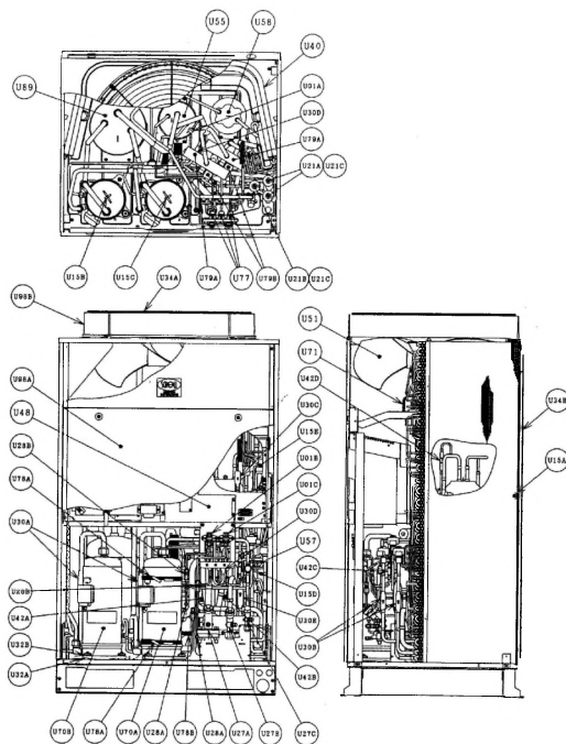
LOCATION OF SPARE PARTS IN THE UNIT A MODEL: RAS-10FXG
