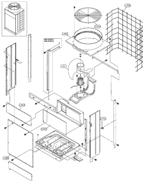
CABINET AND FAN
