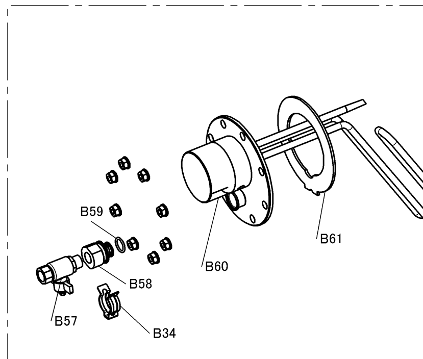
< BOOSTER HEATER >
