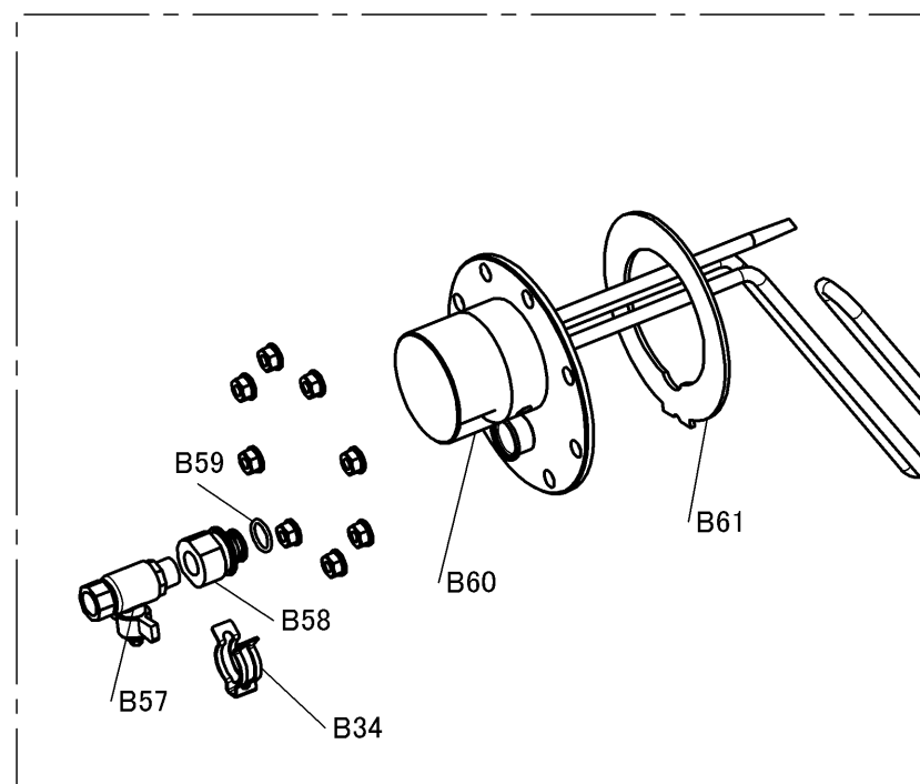
< BOOSTER HEATER >
