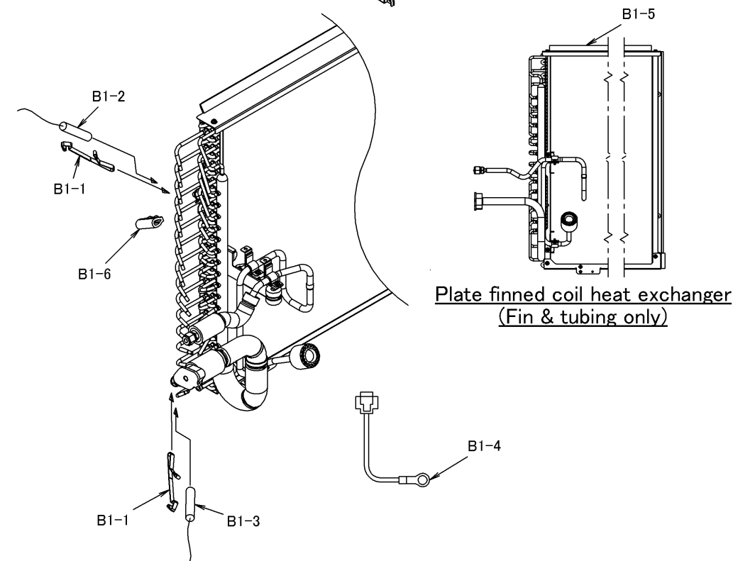
Item ① : Plate finned coil heat exchanger assy
