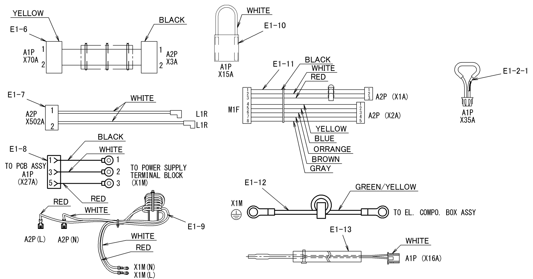
Wire Harness inside electrical component box.
