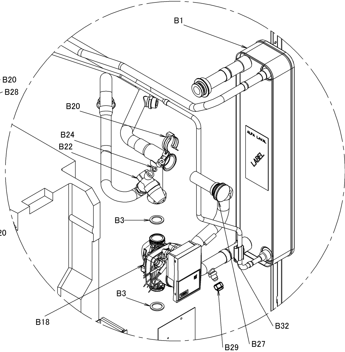
VIEW A
