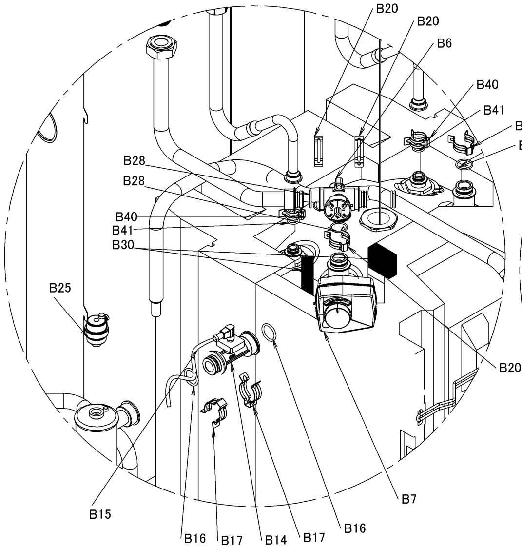
VIEW B
