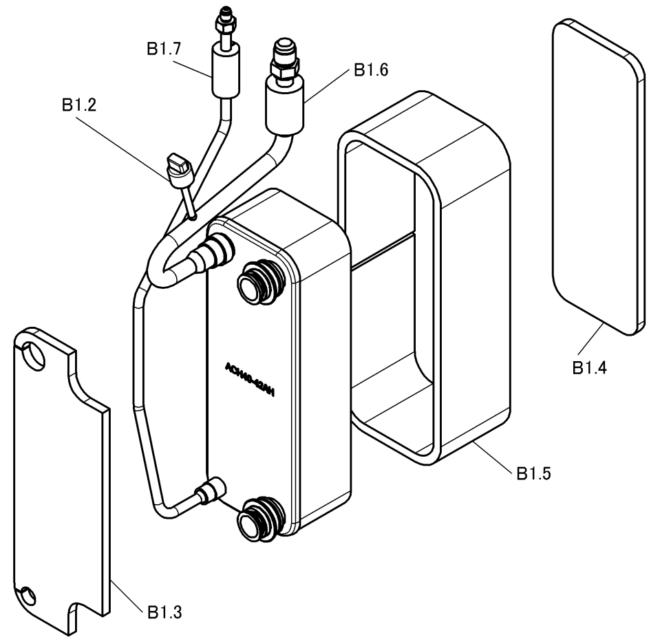
< PLATE HEAT EXCHANGER ASSY >
