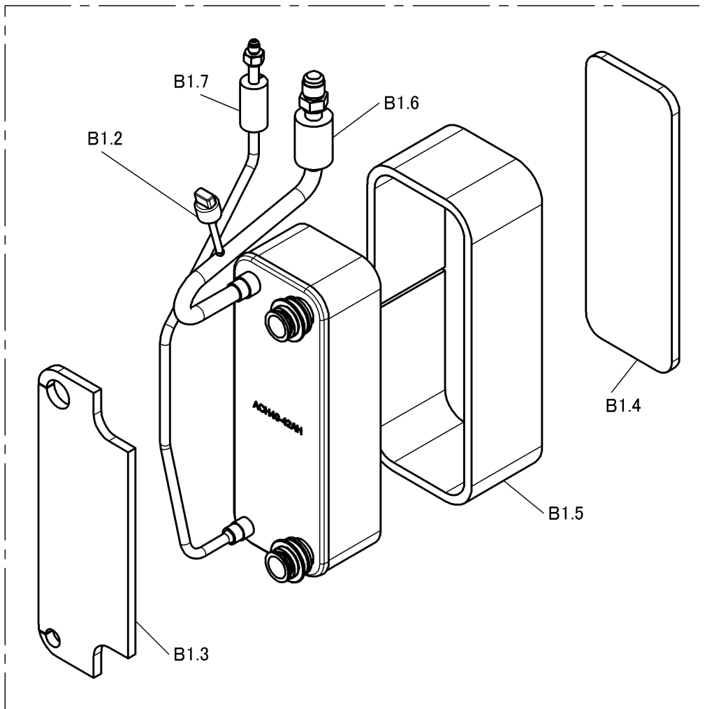
< PLATE HEAT EXCHANGER ASSY >
