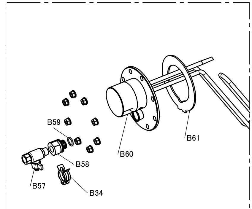
< BOOSTER HEATER >
