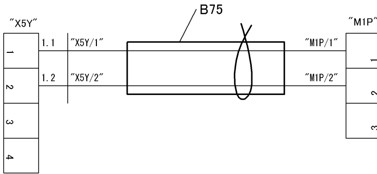
< WIRE HARNESS PUMP (SIGNAL) >
