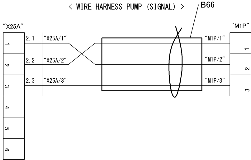
< WIRE HARNESS PUMP (SIGNAL) >
