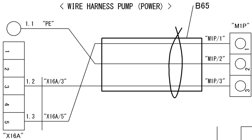
< WIRE HARNESS PUMP (POWER) >
