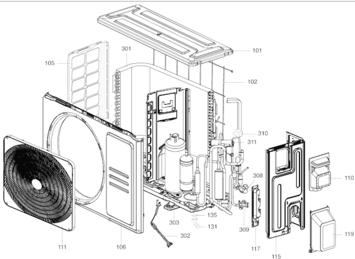
MONO R32 C 70 MD0-O
