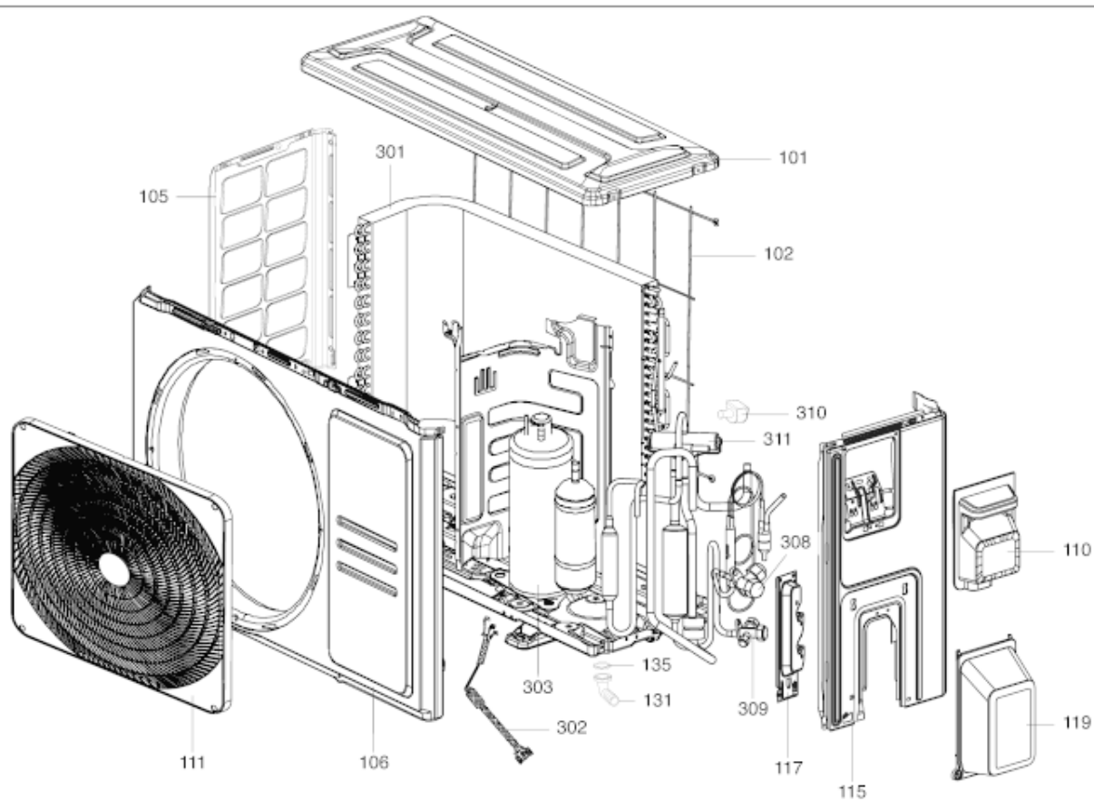
MONO R32 C 50 MD0-O
