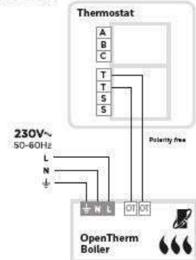
OpenTherm Boiler
