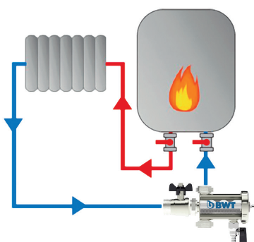
Montage vertical
